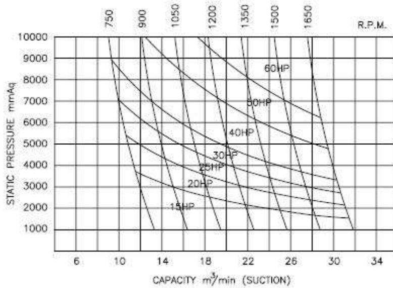
LT-150 PERFORMANCE CURVE
